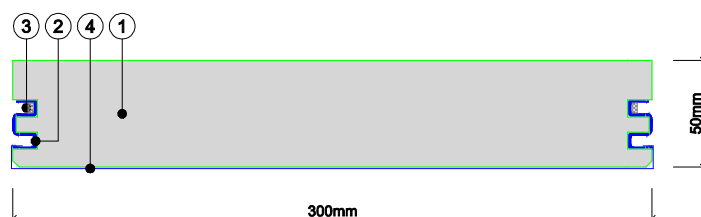
Panel F30 uno + metall 1800x300x50mm
