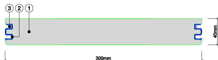
Panel F30 uno 1800x300x40mm
